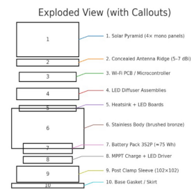
Exploded View
